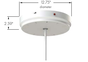
Larger Ceiling Canopy Provided for Model with Emergency IEM Option
